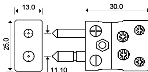
FAR042/0613 ANSI Standard Quick Wire Plugs
