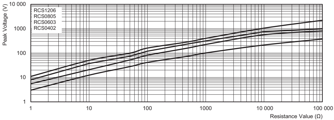
Pulse load rating in accordance with EN 60115-1, 4.27; 10 μs/700 μs; 10 pulses at 1 min intervals; for permissible resistance change 1 %
