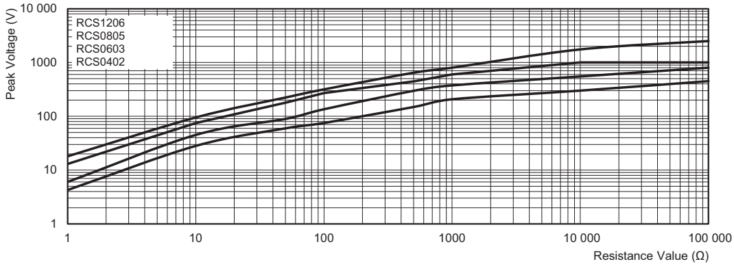
Pulse load rating in accordance with EN 60115-1, 4.27; 1.2 μs/50 μs; 5 pulses at 12 s intervals; for permissible resistance change 1 %
