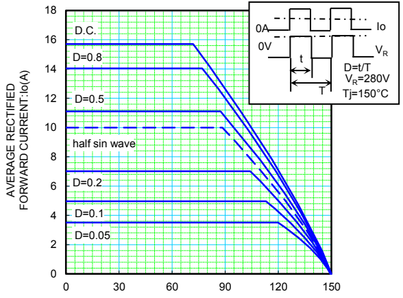
CASE TEMPERATURE: T_c(^{\circ}C) DERATING CURVE ( i_o-T_c )
