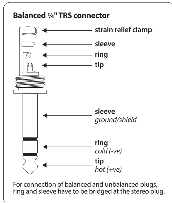
1/4" stereo plug
