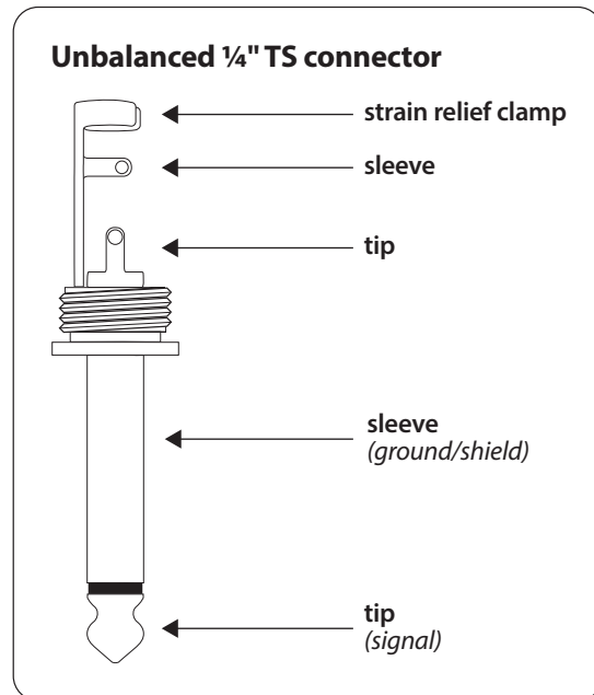
1/4" mono plug
