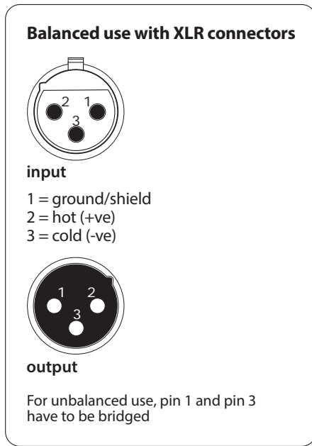
XLR connections
