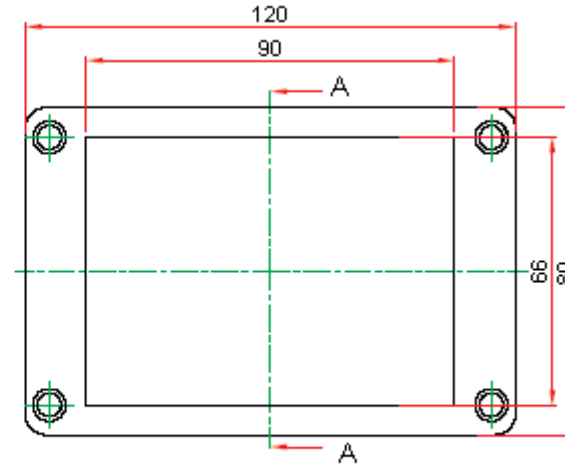
View of Lid
