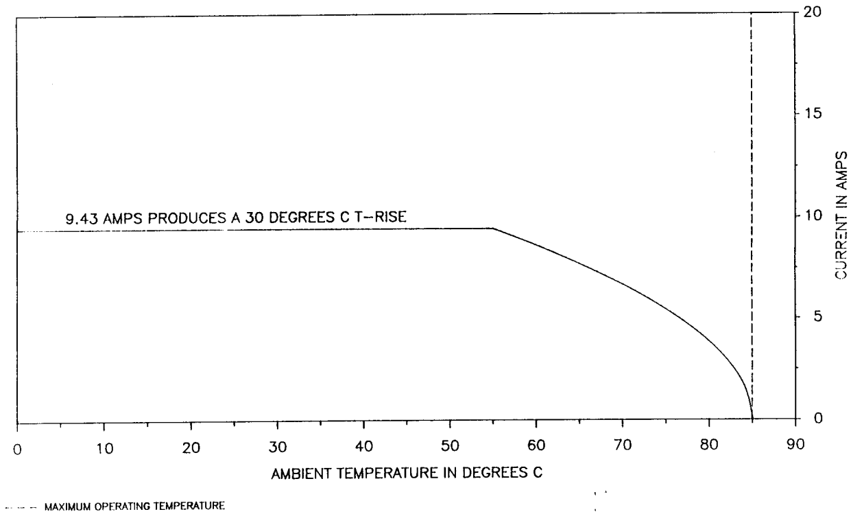
Figure 4A Current Carrying Capacity
