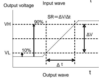
Figure 53. Slew Rate Input Waveform
