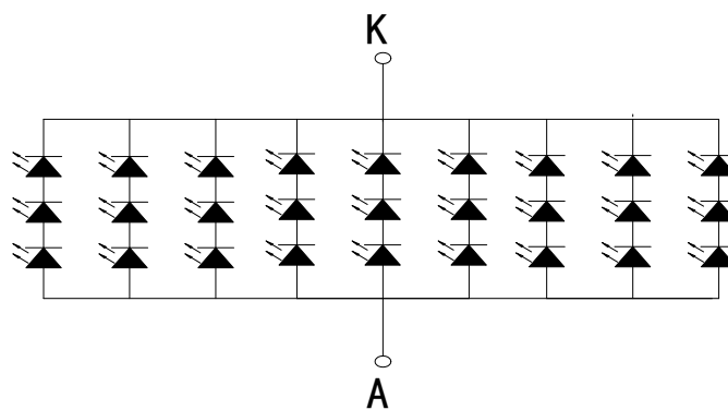
Backlight Circuit diagram
