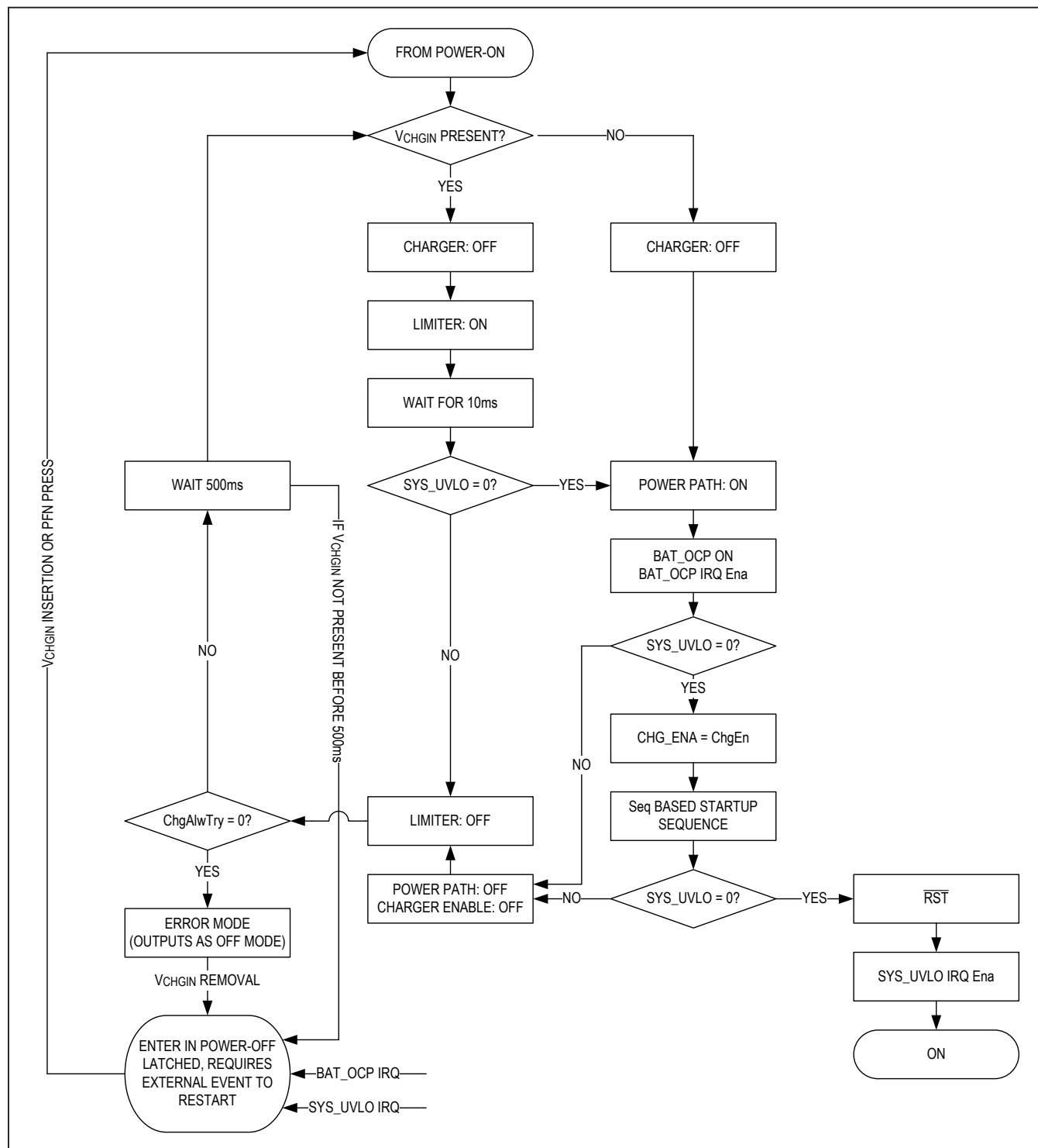
Figure 2. The MAX20345 Boot Sequence
