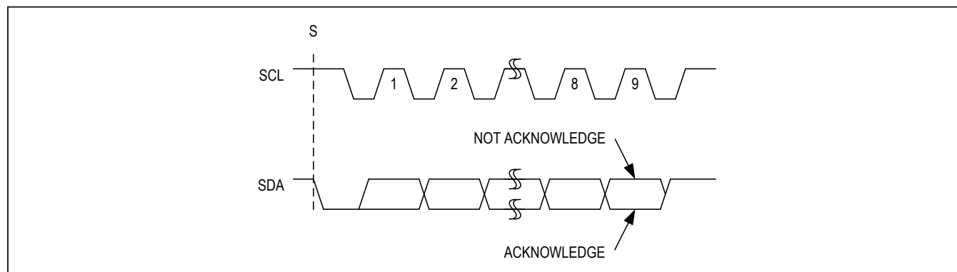
Figure 19. Acknowledge Bits
