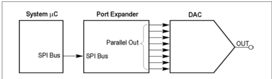
Figure 50. Mixed signal chain block diagram.
