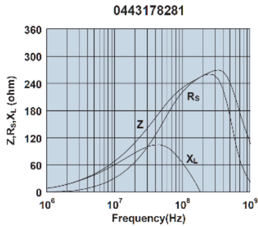
Impedance, reactance, and resistance vs. frequency.
