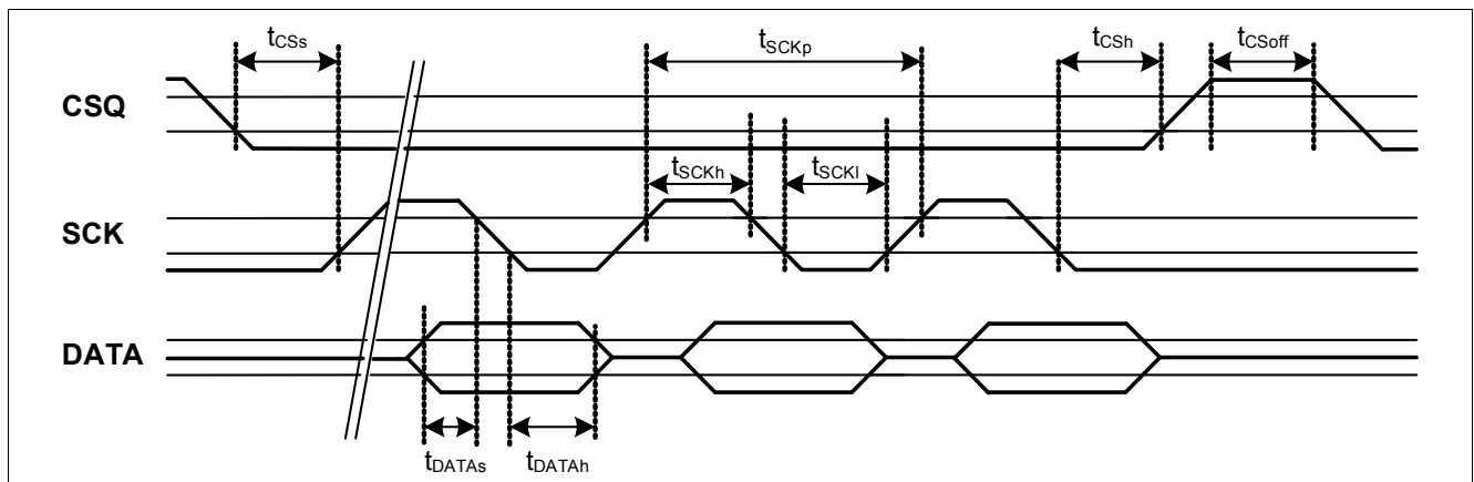
Figure 5-1 SSC timing
