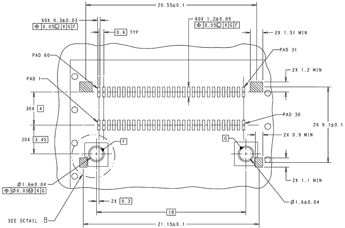
Detail A
