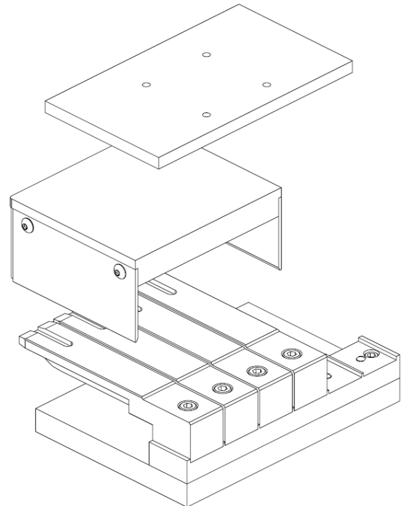
Typical Extraction Tool Kit (Refer to Table)
