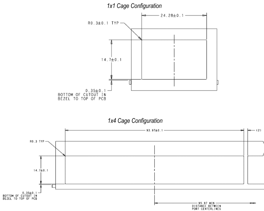
Recommended Bezel Cutout and Minimum Pitch
