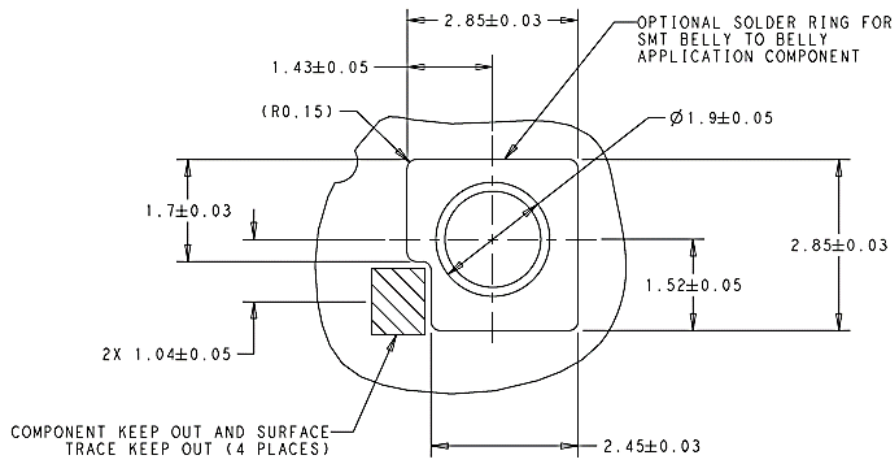
Detail B
