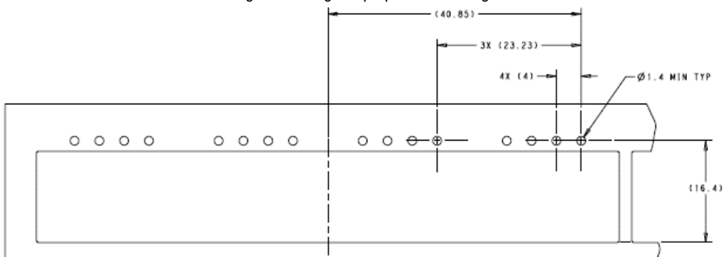
1x4 Cage with 4 Light Pipe per Port Configuration
