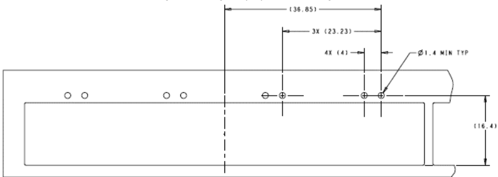
1x4 Cage with 2 Light Pipe per Port Configuration
