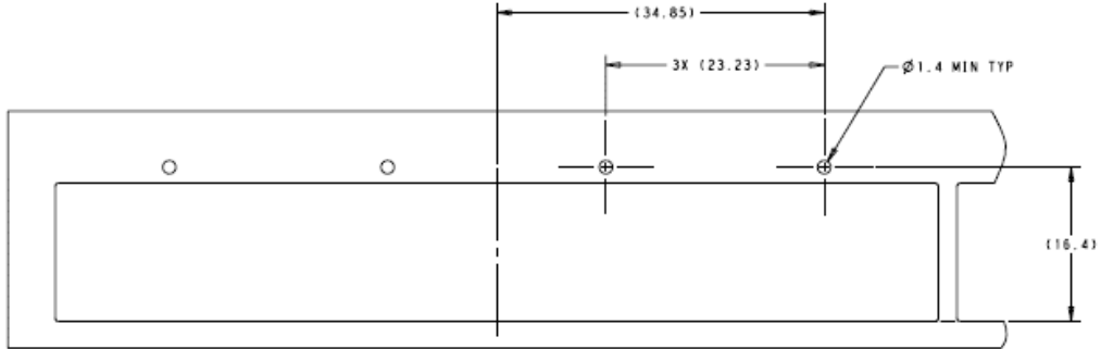
1x4 Cage with 1 Light Pipe per Port Configuration
