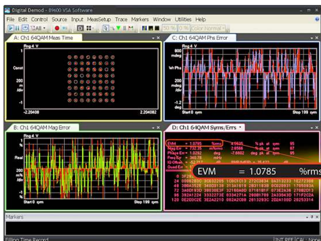
Figure 5. Constellation diagram and EVM of 64-QAM baseband signal with added noise
