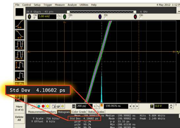
Figure 1. Jitter measurement on the 33522A waveform generator
