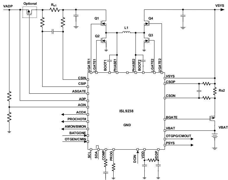
FIGURE 1. BLOCK DIAGRAM
