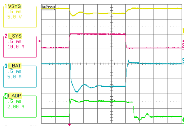
FIGURE 13. BOOST MODE, OUTPUT VOLTAGE LOOP TO ADAPTER CURRENT LOOP TRANSITION. V_{ADP} = 5V , MAXSYSTEMVOLTAGE = 8.496V, V_{BAT} = 7V , SYSTEM LOAD 0.5A TO 10A STEP, ADAPTERCURRENTLIMIT = 3A, CHARGECURRENT = 0A
