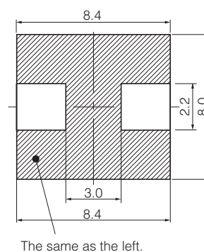
Series PCC-M0748M-LE (ETQP4M□□□KFM)
