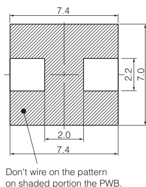
Series PCC-M0648M-LE (ETQP4M□□□KFN)
