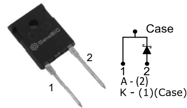
TO-247-2L
