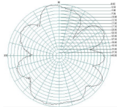
H Plane
