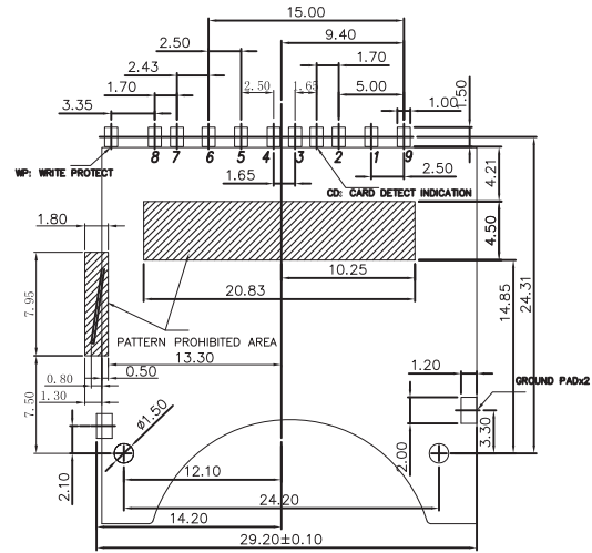
PCB LAYOUT - COMPONENT VIEW TOLERANCES: ±0.05
