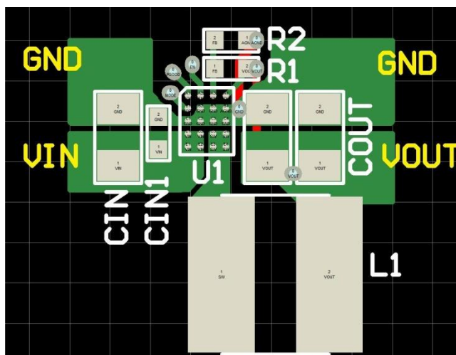
Figure 28. Recommended Layout
