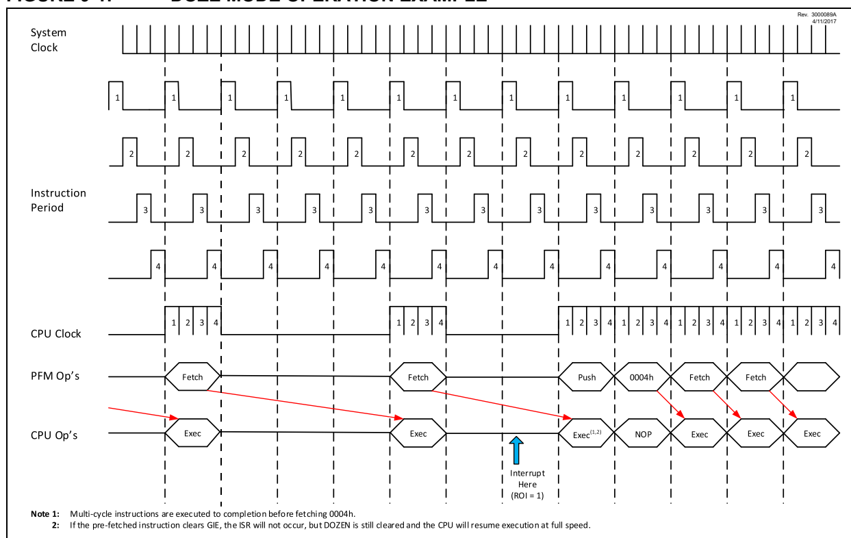
FIGURE 9-1: DOZE MODE OPERATION EXAMPLE
