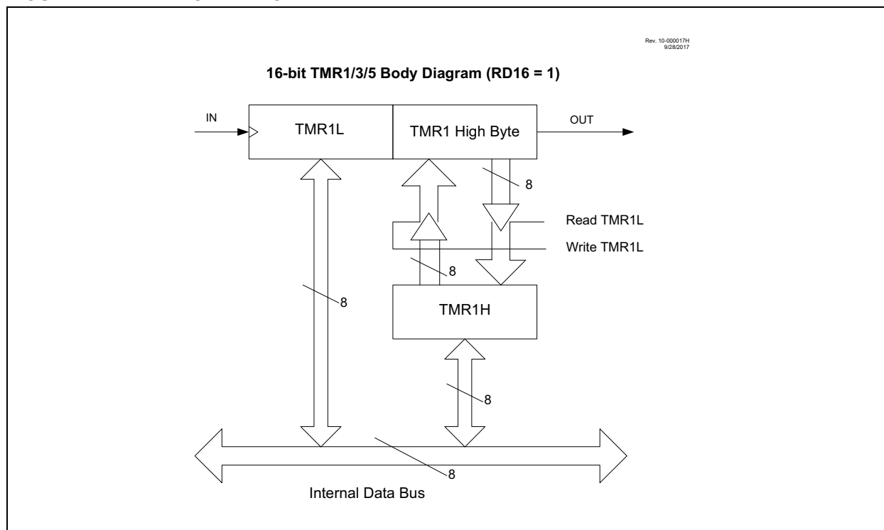
FIGURE 27-2: BODY DIAGRAM
