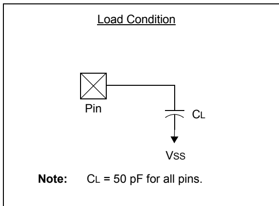
FIGURE 35-4: LOAD CONDITIONS
