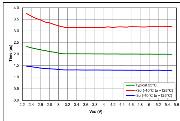
FIGURE 36-70: ADC RC Oscillator Period (PIC16F18326/46 only)
