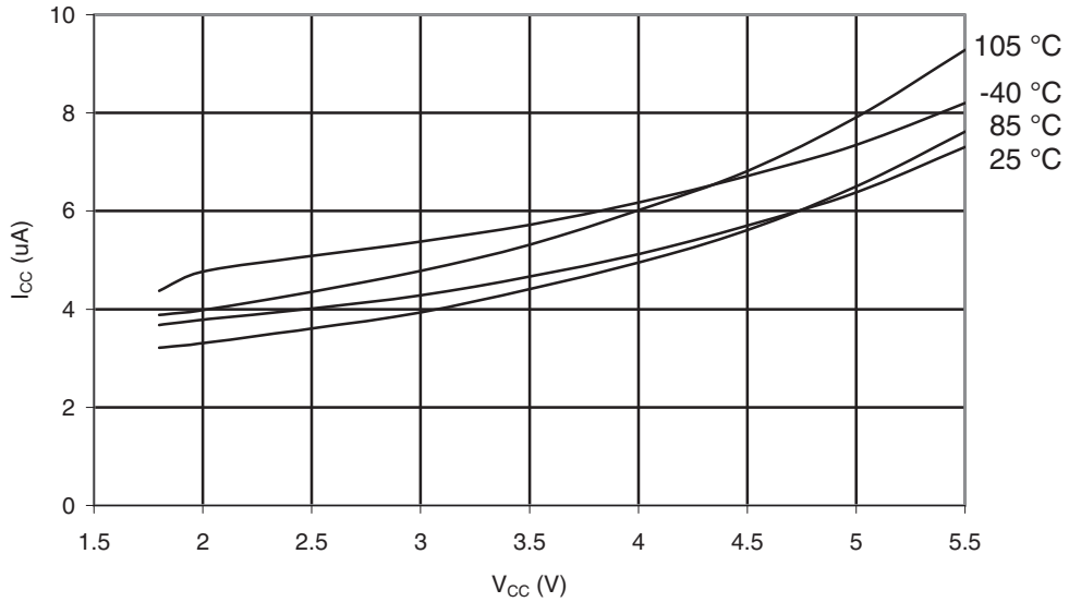
Figure 31-49. Power-down Supply Current vs. V_{CC} (Watchdog Timer Enabled)
