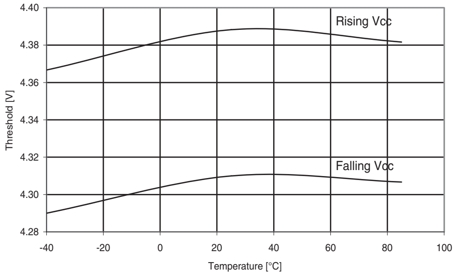
Figure 30-129. ATmega324A: BOD threshold vs. temperature ( V_{BOT} = 4.3V )
