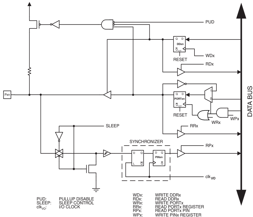
Note: 1. WRx, WPx, WDX, RRx, RPx, and RDx are common to all pins within the same port. clk I/O , SLEEP, and PUD are common to all ports.
