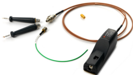
Figure 4. N7024A power rail probe and included accessories, N7021A coaxial "pigtail" probe heads, N7022A main cable, N7023A browser (not shown), N7032A 4GHz browser, N7033A 5GHz browser and rotating SMA adapter.
