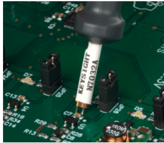
Figure 18. Close up view of the N7032A 4GHz power rail probe browser probing a small capacitor package on the power distribution network
