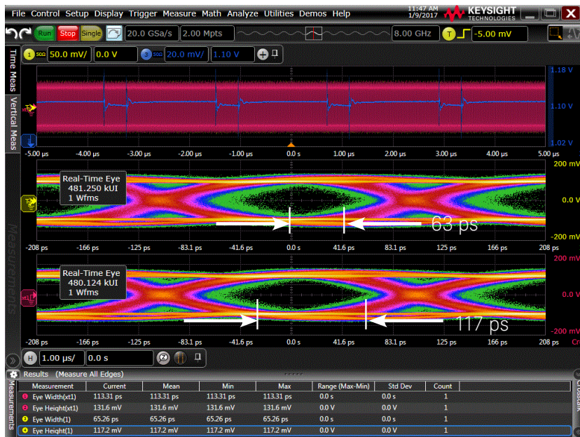
Figure 26. Results from the D9010POWA PI analysis application showing the eye diagram of the FPGA serial data before and after the effects of the DC supply noise are removed. Notice that the results are nearly identical to the previous results where the supply was physically change to
