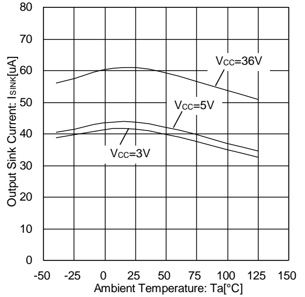
Figure 11. Output Sink Current vs Ambient Temperature (V OUT =0.2V)
