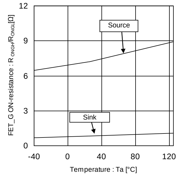
Figure 21. FET_G ON-resistance vs Temperature (Source /Sink)
