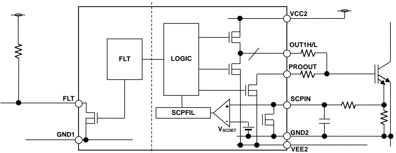
Figure 8. Block Diagram of Short Circuit Protection
