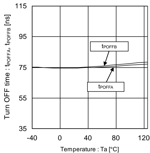
Figure 37. Turn OFF time vs Temperature
