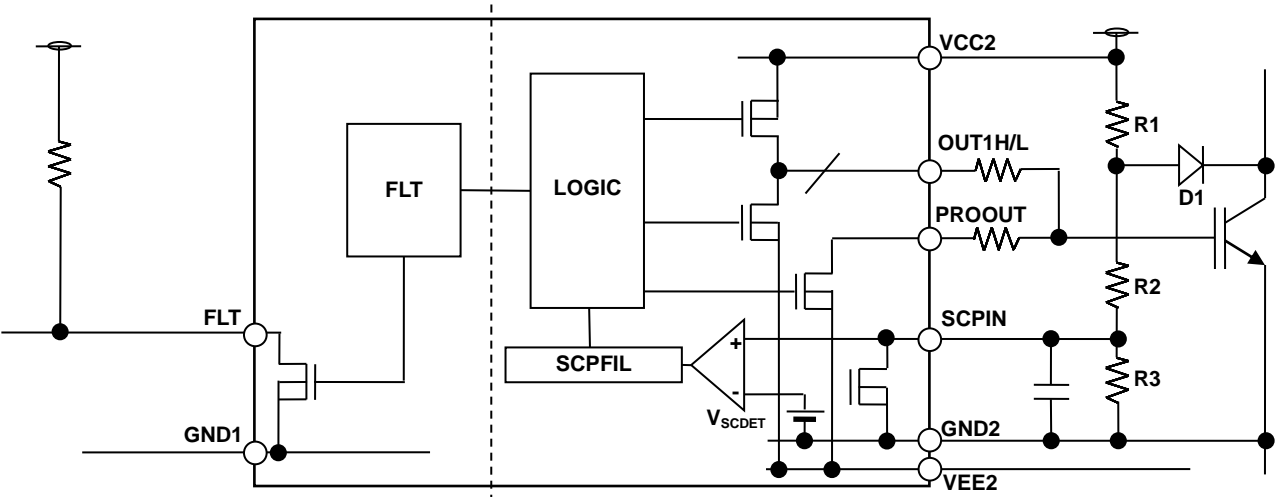
Figure 9. Block Diagram of DESAT
