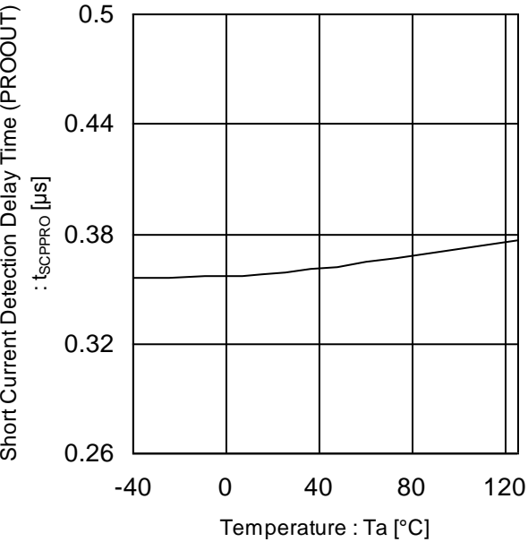
Figure 42. Short Current Detection Delay Time (PROOUT) vs Temperature
