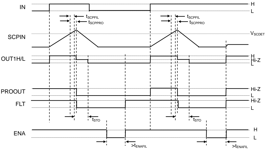
Figure 10. SCP Operation Timing Chart
