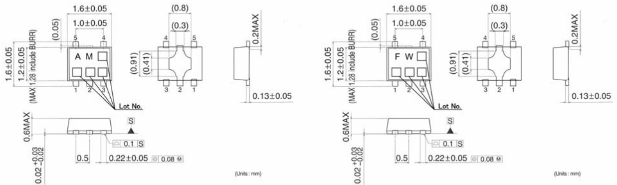
BU7465HFV (HVS0F5) (Unit : [mm])
