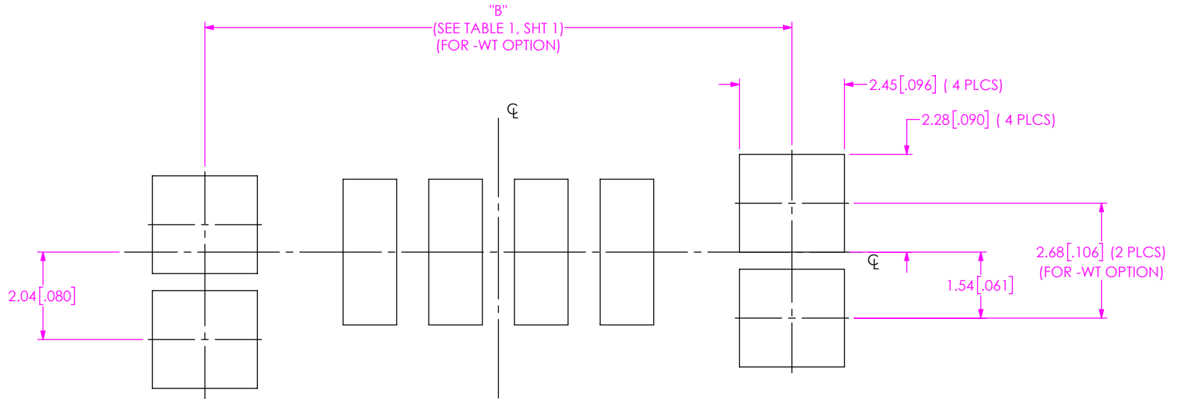
FIG 2 UMPT-04-XX.X-X-VT-SM-X-WT STENCIL SHOWN A (DIFFERENT AS SHOWN, OTHERWISE SAME AS FIG 1)
