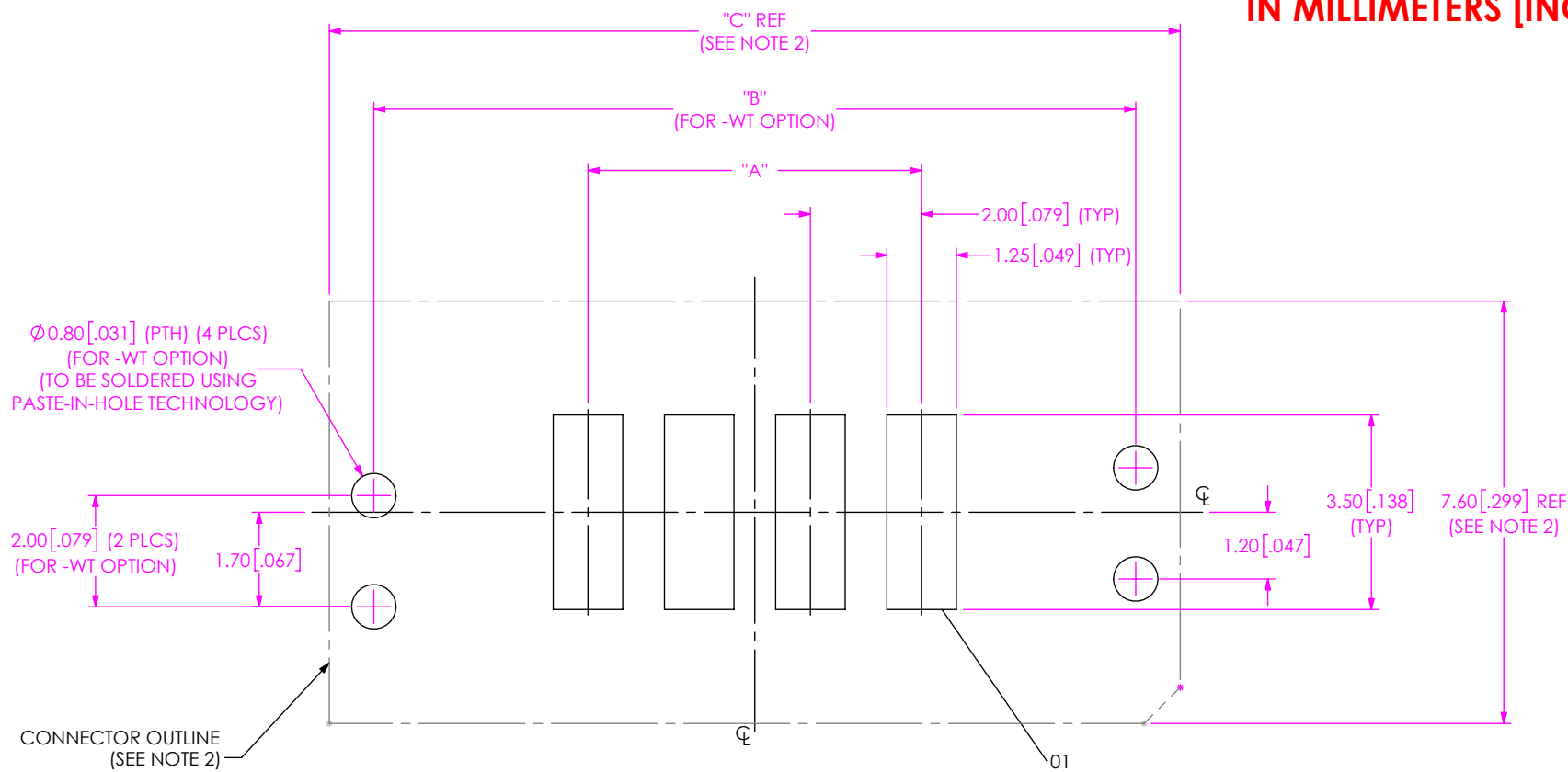
FIG 1 UMPT-04-XX.X-X-VT-SM-X-WT FOOTPRINT SHOWN
