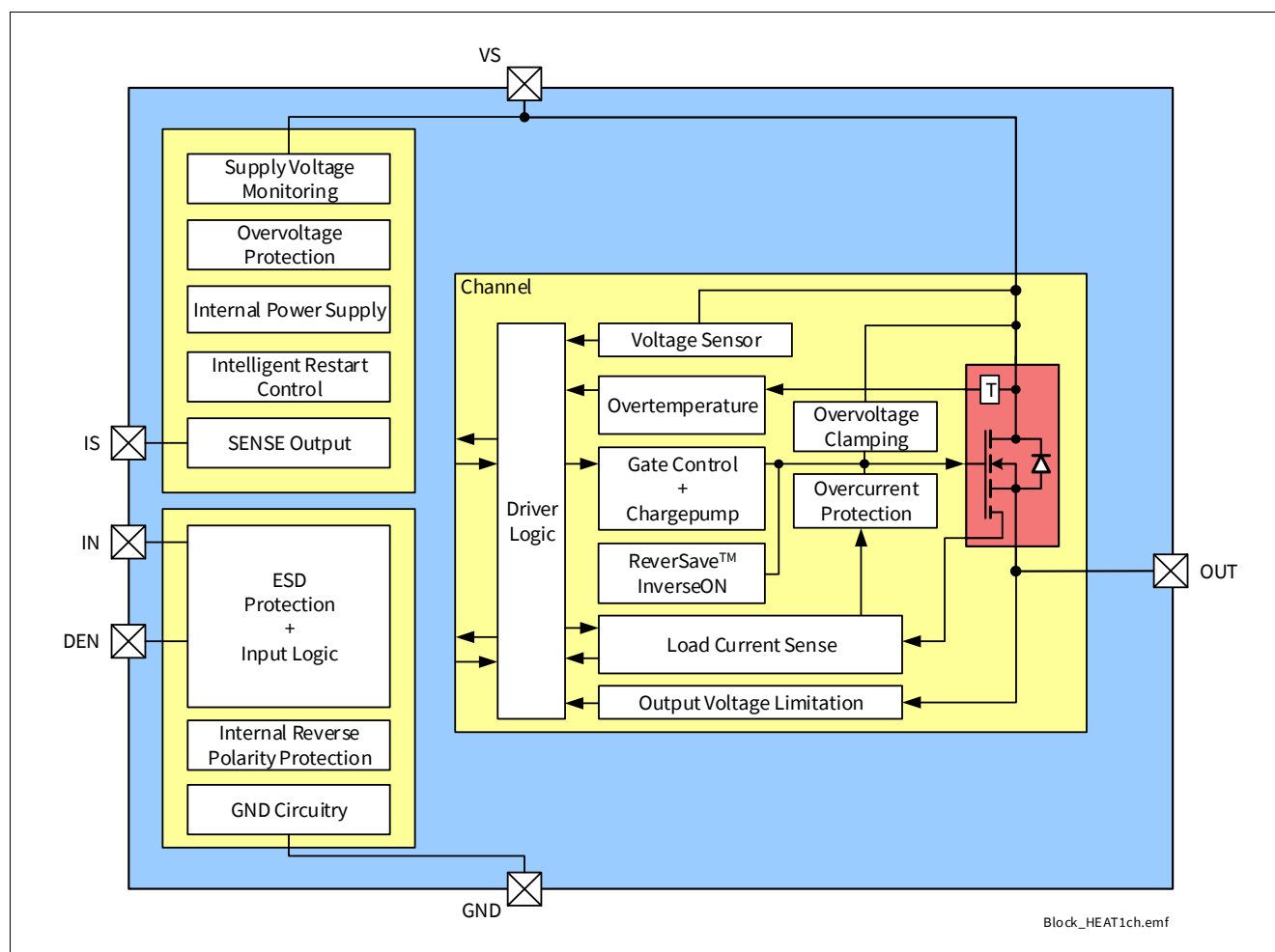
Figure 2 Block Diagram of BTS7006-1EPP
