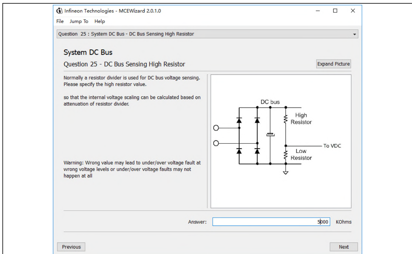
Figure 10 DC bus sensing configuration in MCEWizard
