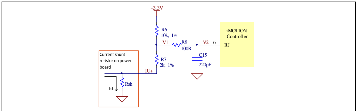
Figure 12 The part of Current feedback on the EVAL-M1-101T evaluation board
