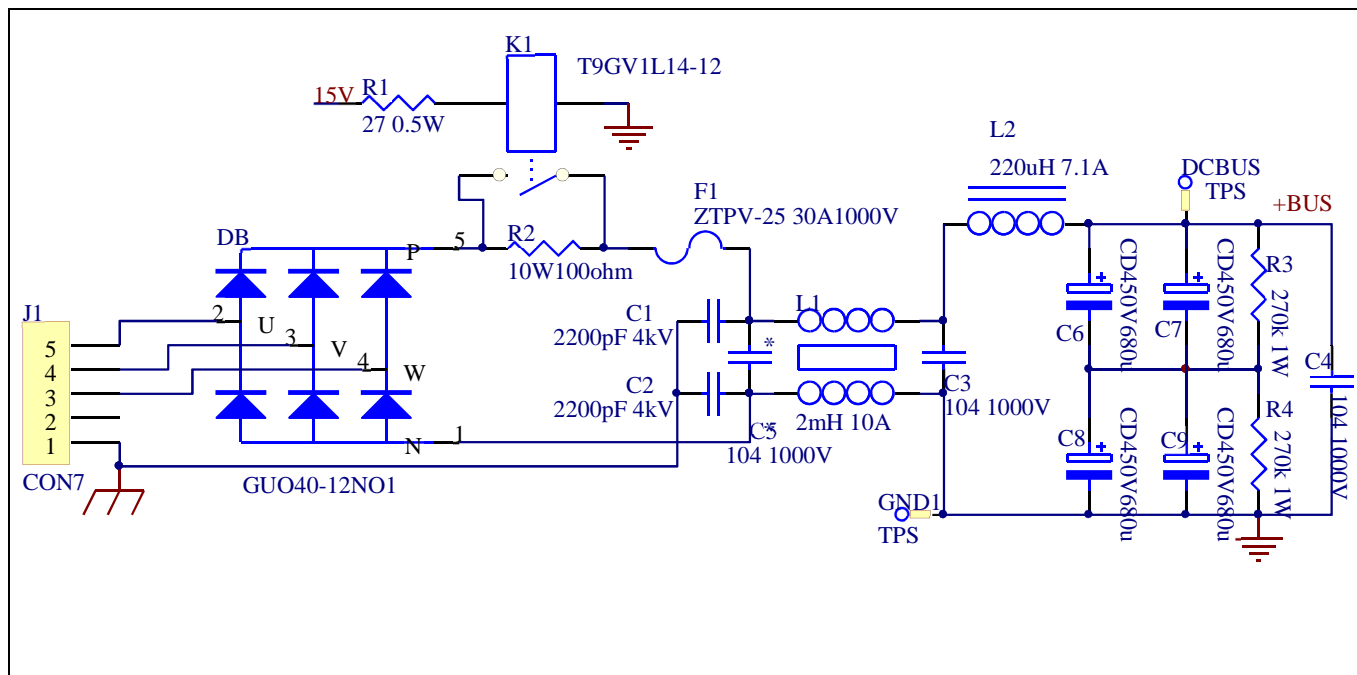
Figure 14 Schematic for EMI filter and AC/DC section of the EVAL-M1-IM818-A evaluation board
