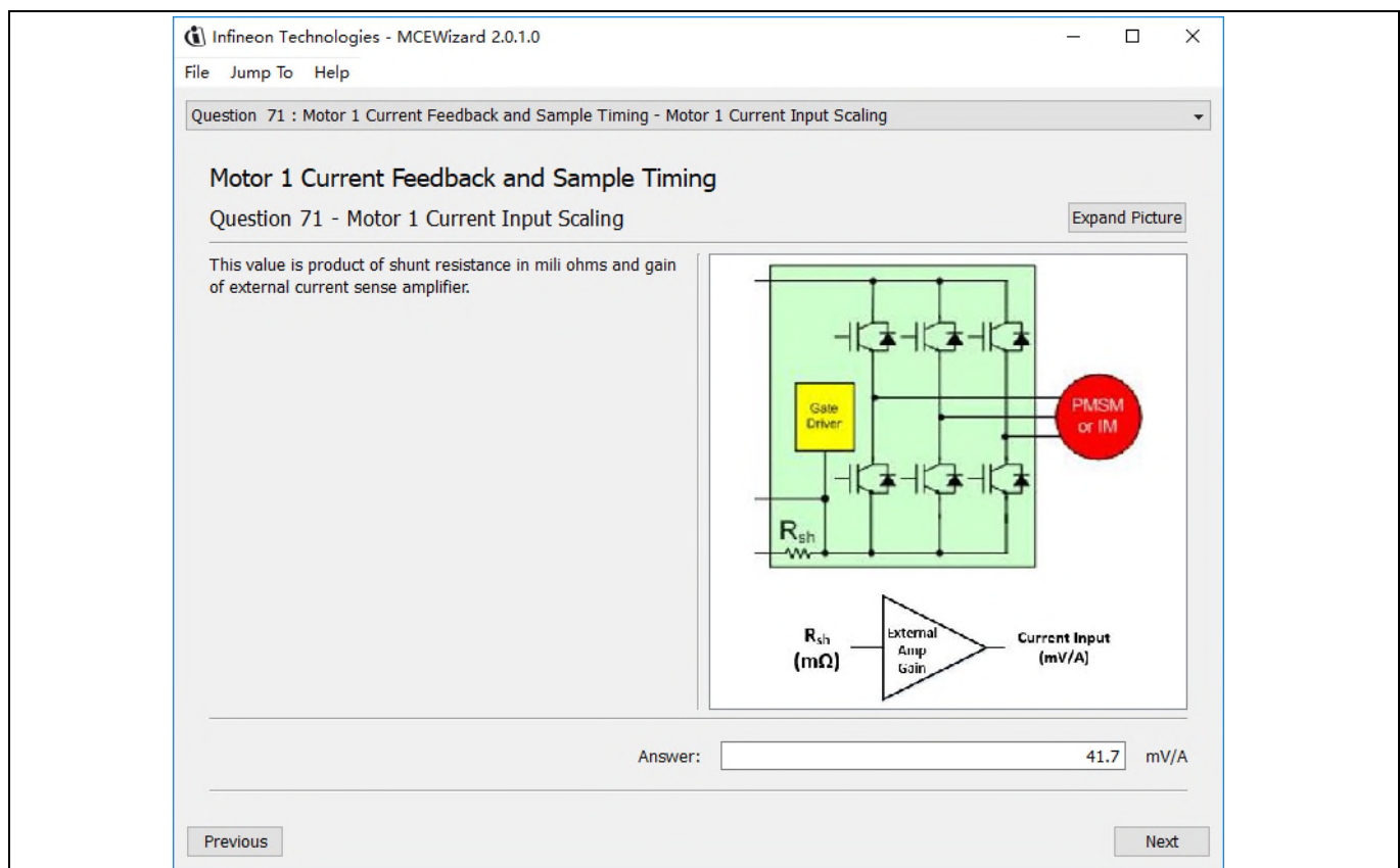
Figure 13 Current feedback configuration in MCEWizard for EVAL-M1-101T and EVAL-M1-IM818-A
