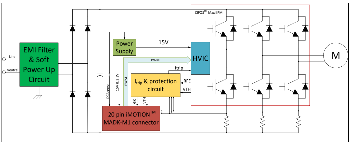
Figure 1 The Block Diagram of the EVAL-M1-IM818-A
