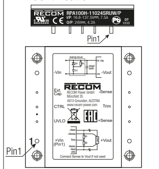
Pin1 identification
