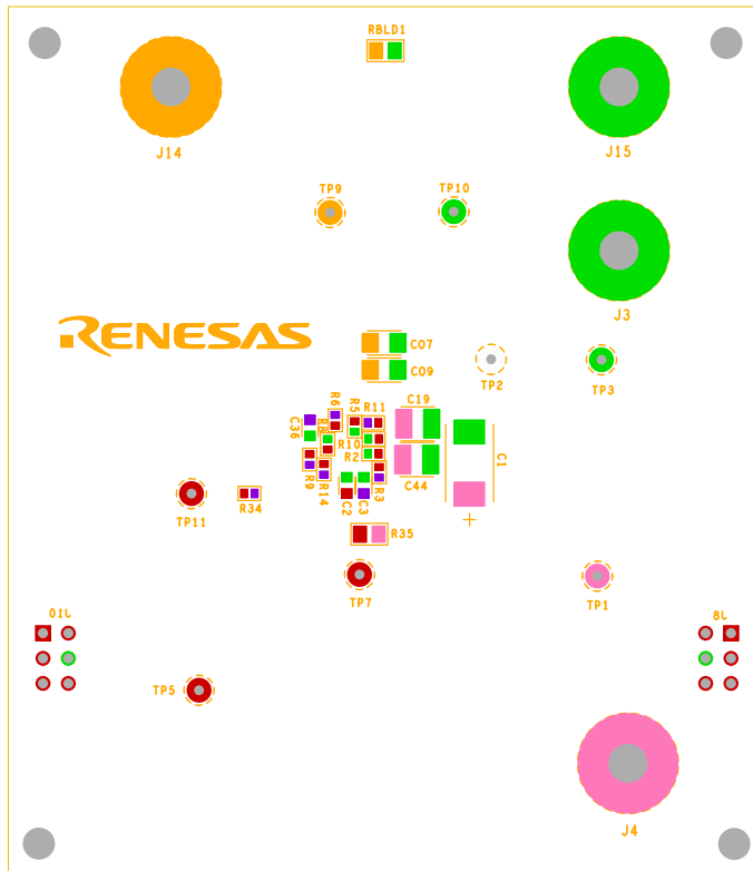
Figure 14. Silkscreen Bottom
