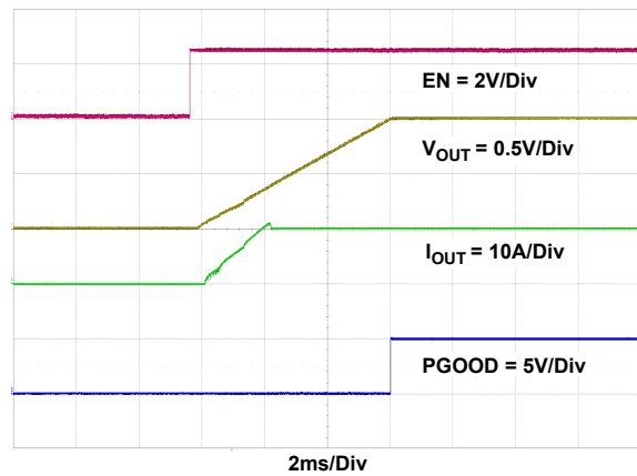
Figure 22. Startup Waveform at I_{OUT} = 10A
