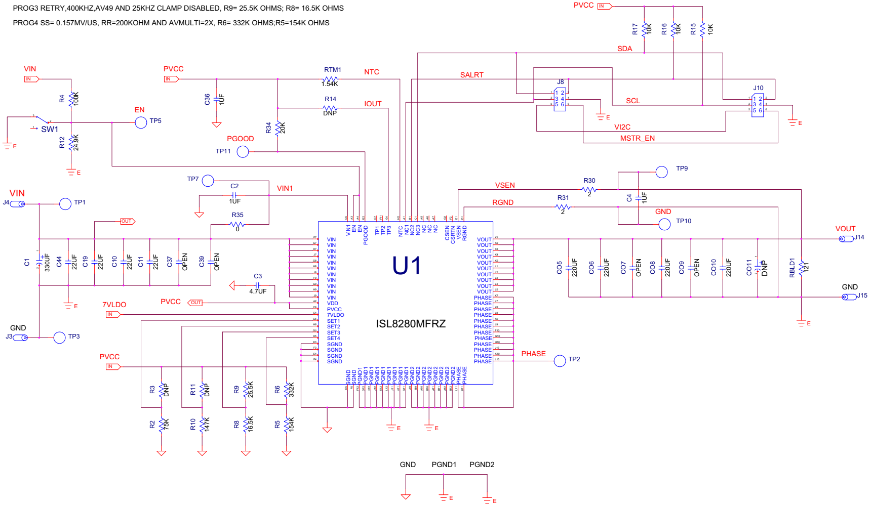
Figure 6. Schematic
