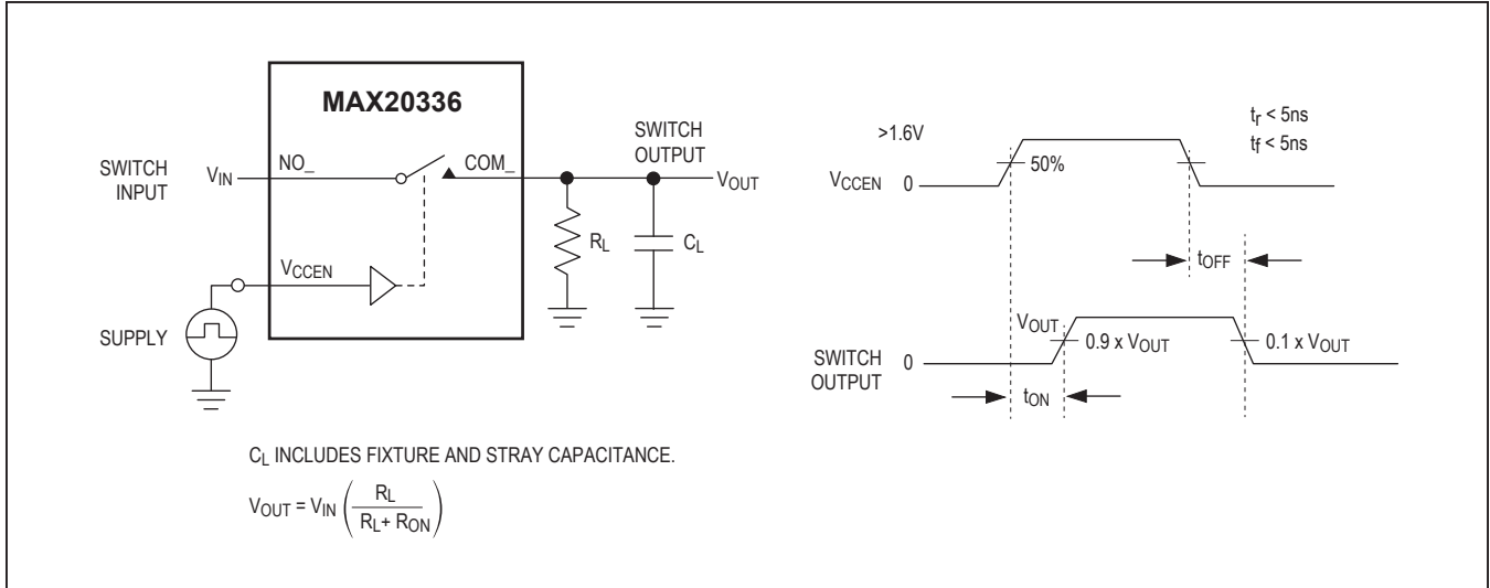
Figure 1. Switching Time
