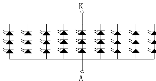
Figure : LED connection of backlight
