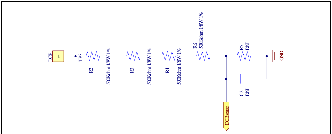
Figure 11 DC bus sense resistor on EVAL-M1-CTE610N3 evaluation board
