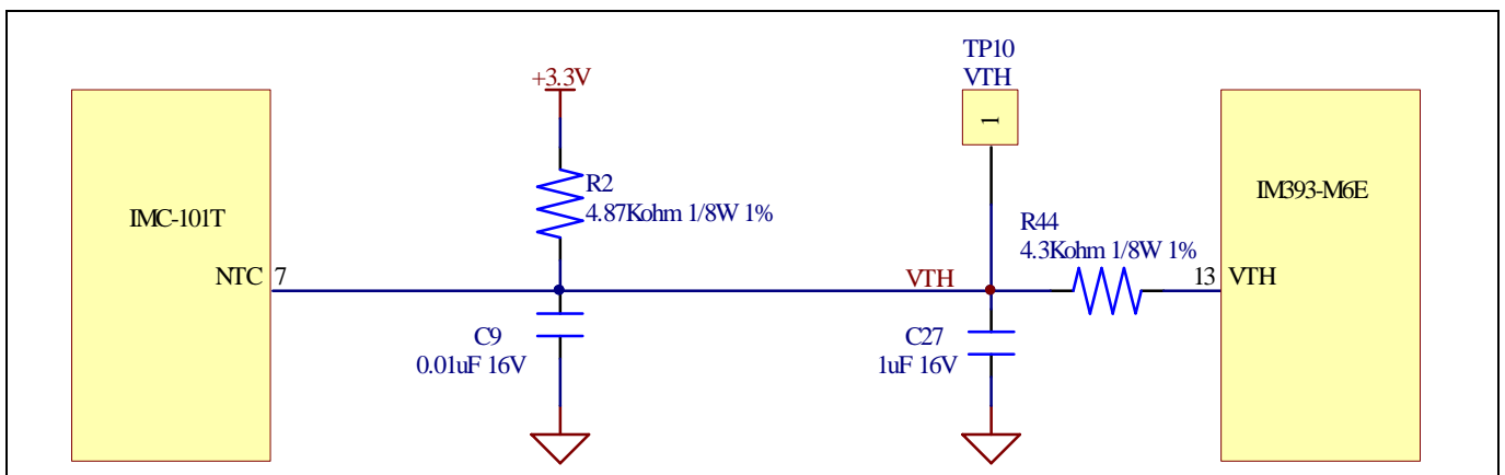
Figure 19 Overtemperature protection circuit schematic for EVAL-M1-CTE610N3 and EVAL-M1-101T
