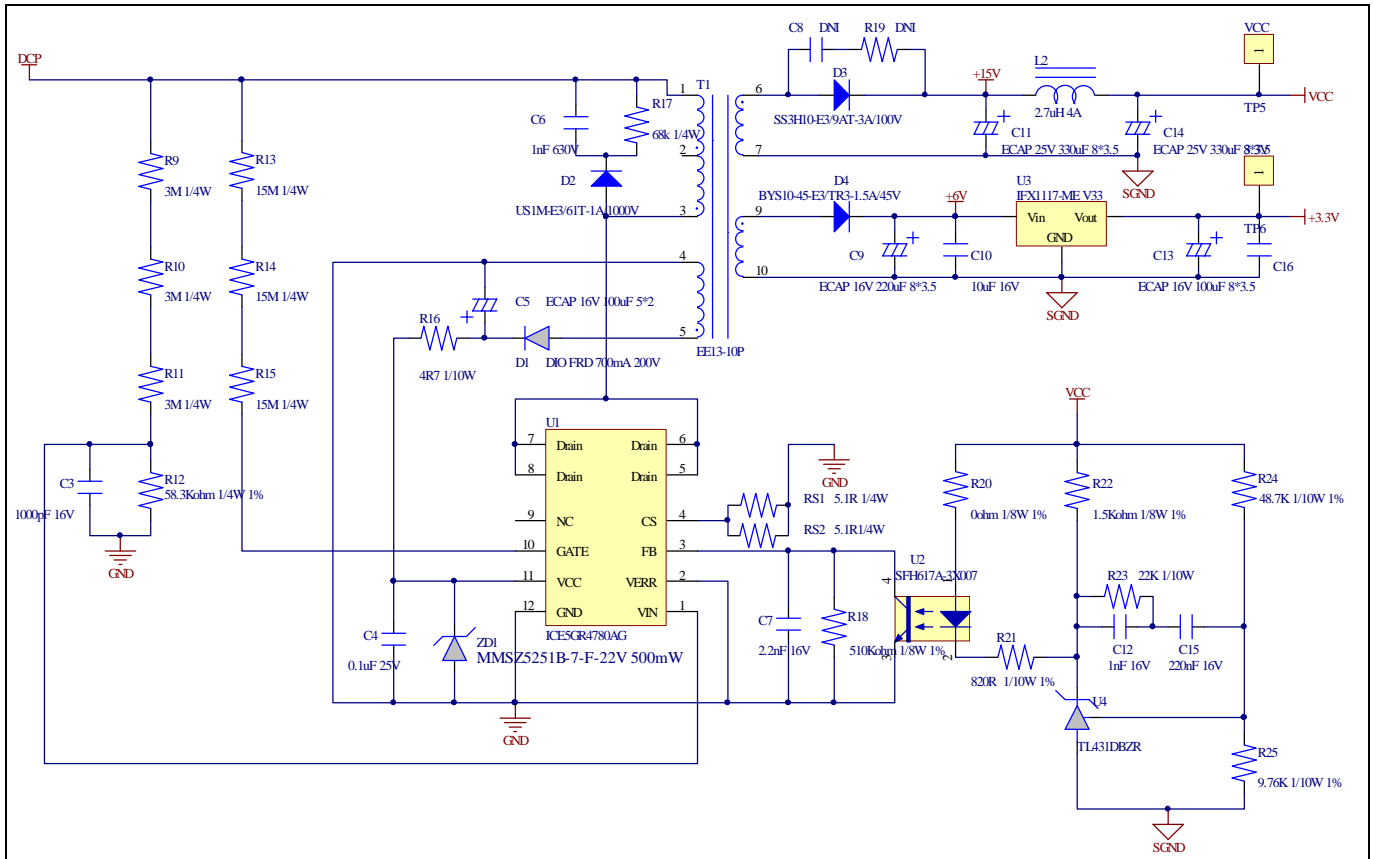
Figure 21 Power supply section of the EVAL-M1-CTE610N3 evaluation board
