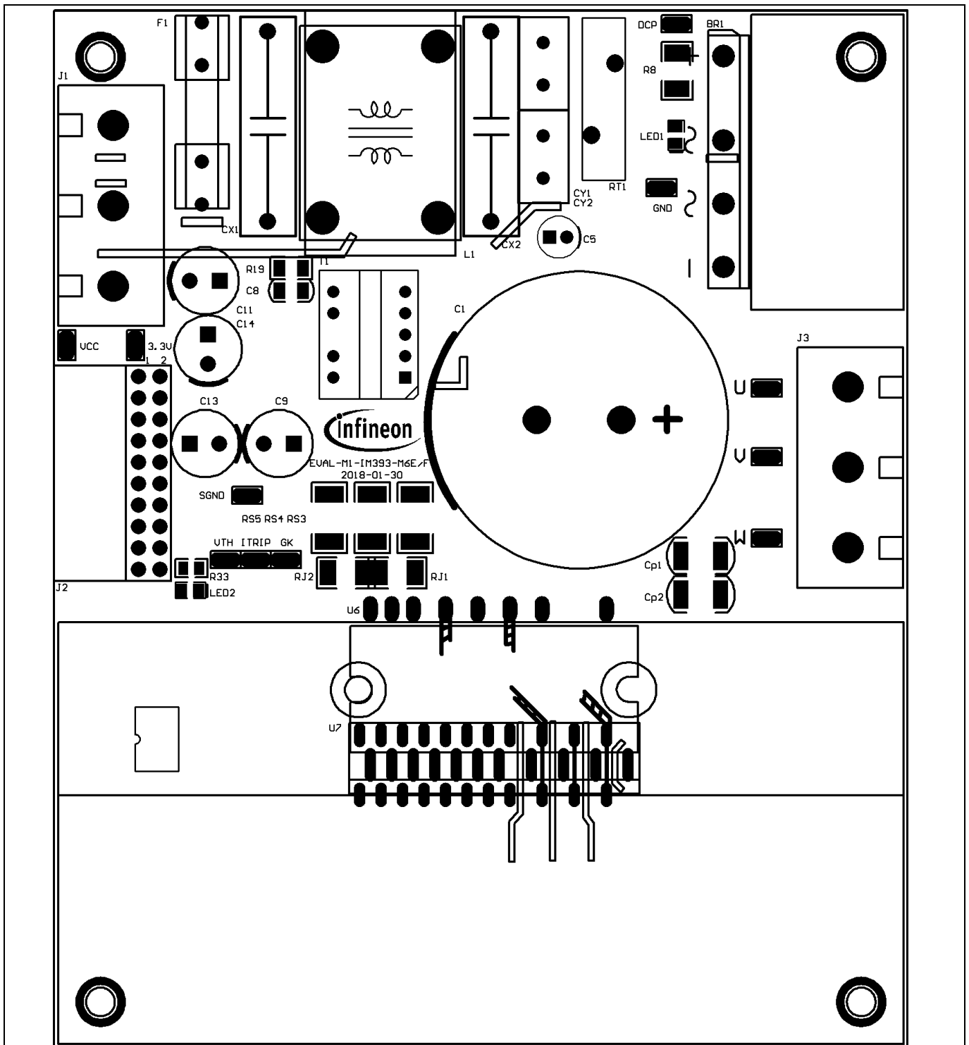
Figure 25 Top assembly print of the EVAL-M1-CTE610N3 evaluation board
