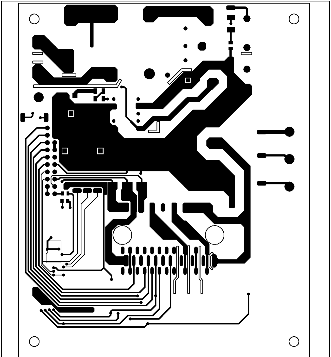
Figure 27 Top layer routing of the EVAL-M1-CTE610N3
