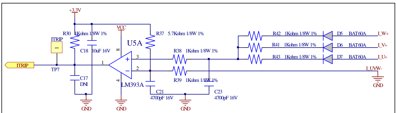
Figure 16 Overcurrent protection circuit on the EVAL-M1-CTE610N3 evaluation board
