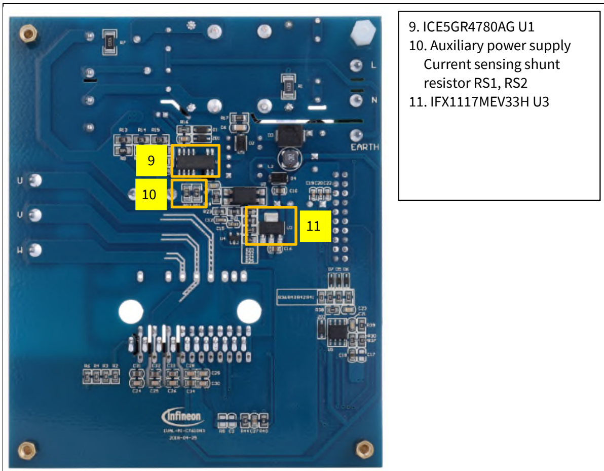
Figure 3 Functional groups of the EVAL-M1-CTE610N3 evaluation board’s bottom side
