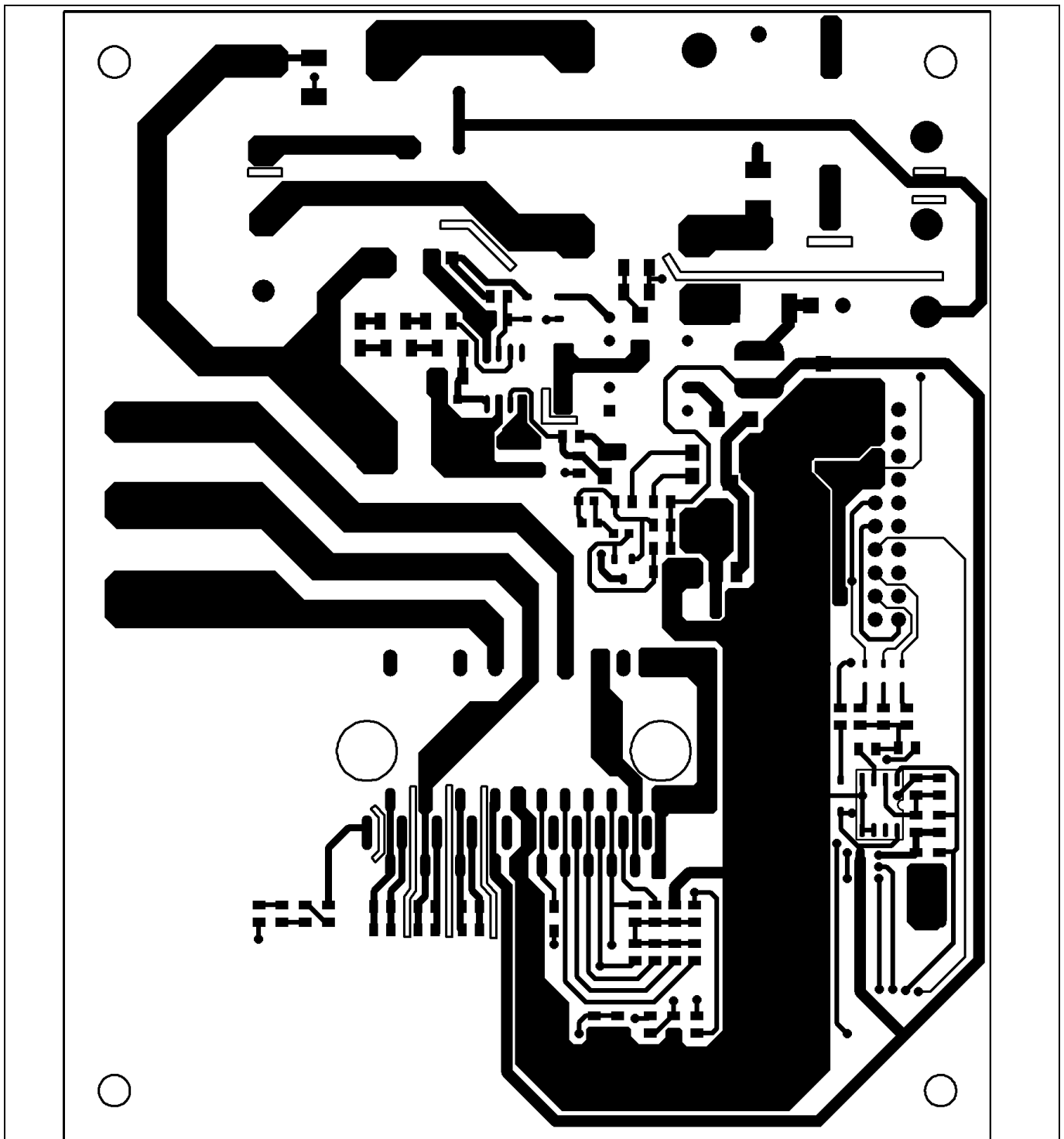
Figure 28 Bottom layer routing of the EVAL-M1-CTE610N3
