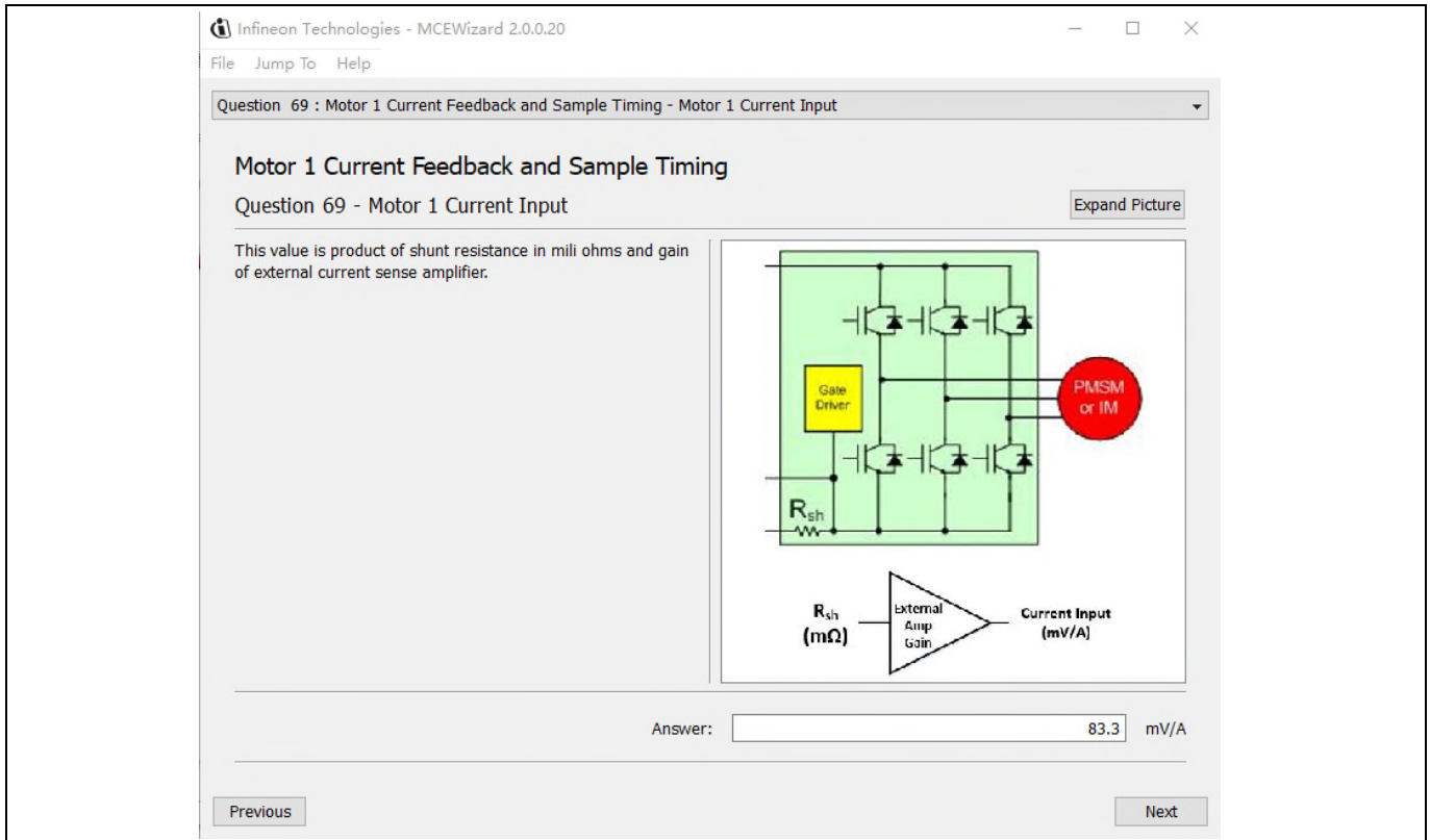
Figure 15 Current feedback configuration in MCEWizard for EVAL-M1-101T and EVAL-M1-CTE610N3
