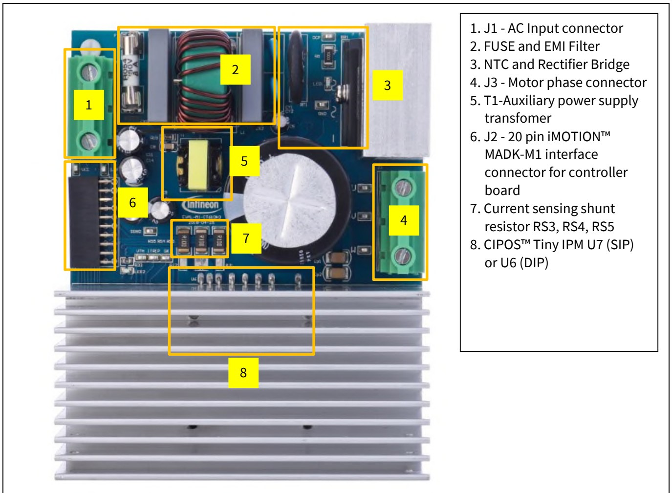
Figure 2 Functional groups of the EVAL-M1-CTE610N3 evaluation board's top side
