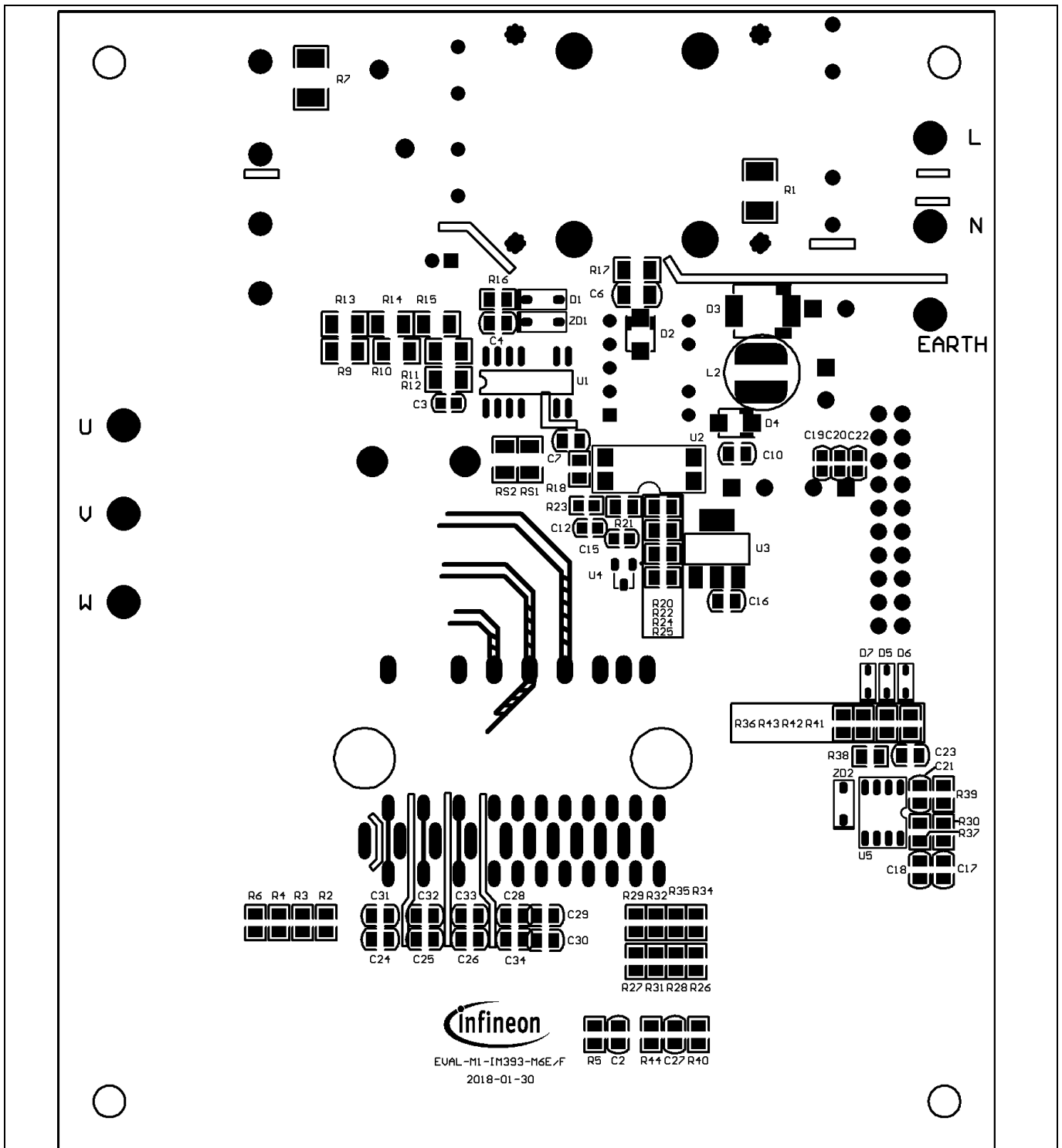
Figure 26 Bottom assembly print of the EVAL-M1-CTE610N3 evaluation board
