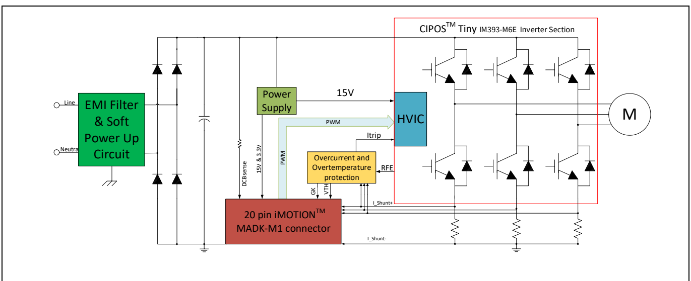
Figure 1 The Block Diagram of the EVAL-M1-CTE610N3
