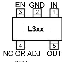
MIC5233 5-Pin SOT23 (Top View)
