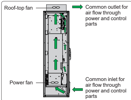
IP 20, 21, 23, 40, 41, 43/Type 1 integration common cooling air flow
