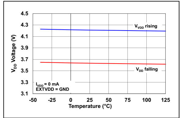
FIGURE 2-10: V_{DD} UVLO Threshold vs. Temperature.
