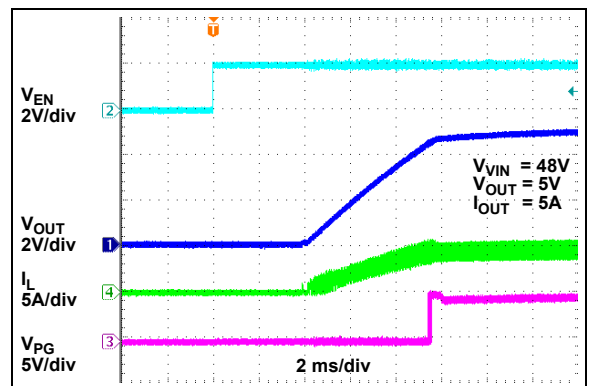
FIGURE 2-36: Enable Turn-On Delay.
