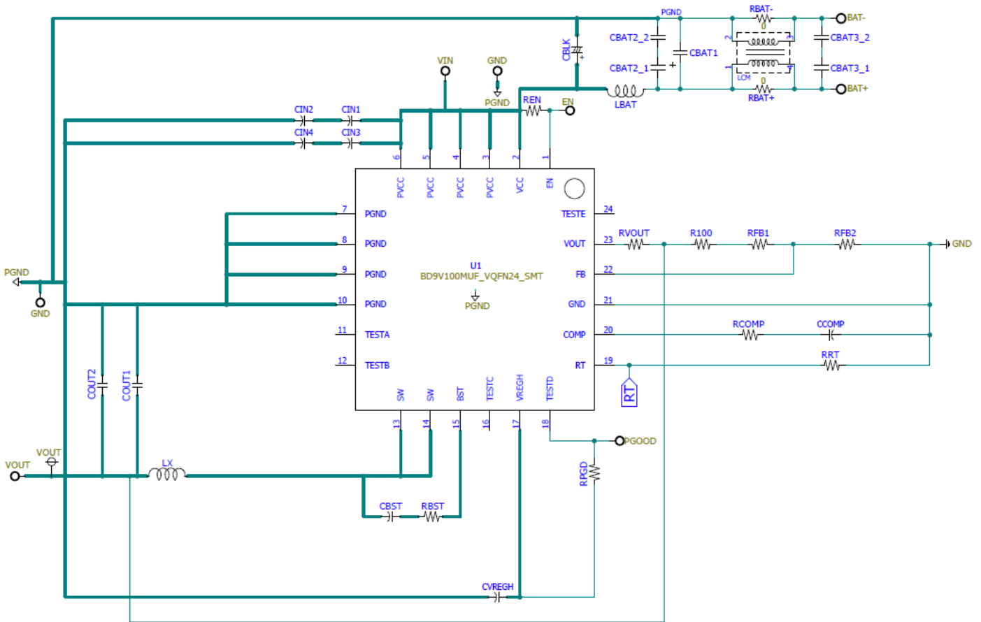
Fig 2: BU33UV7NUX Evaluation Board Schematic
