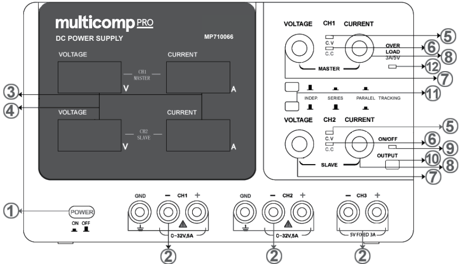
Figure 1 – Front Panel: Models MP710066 / MP710067
