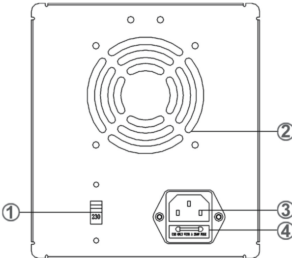
Figure 4 – Rear Panel: Models MP710066 / MP710067
