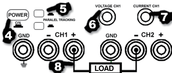
Figure 9 - Parallel Connection of the adjustable power supplies of the MP710066 and MP710067
