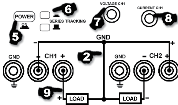
Figure 11 - Symmetric Connection of the adjustable power supplies of the models MP710066 and MP710067.
