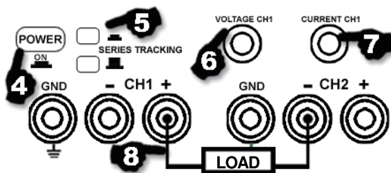
Figure 10 - Series Operation Mode of the adjustable power supplies of the models MP710066 and MP710067.
