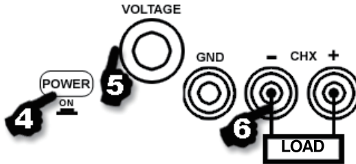
Figure 8 - Models MP710066 and MP710067 Connections
