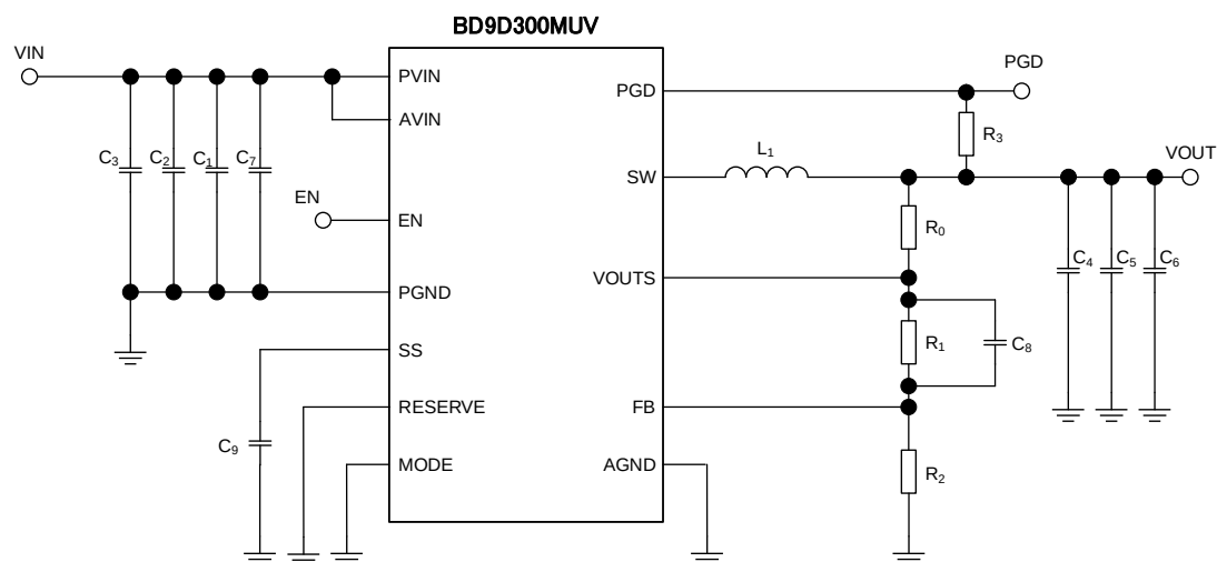
Figure 40. Application Circuit
