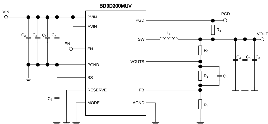
Figure 50. Application Circuit
