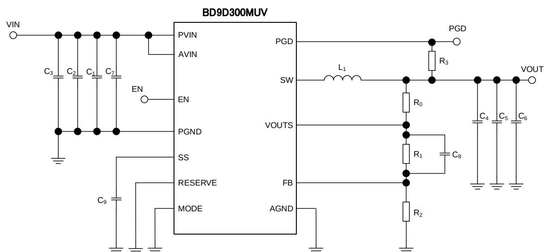
Figure 45. Application Circuit
