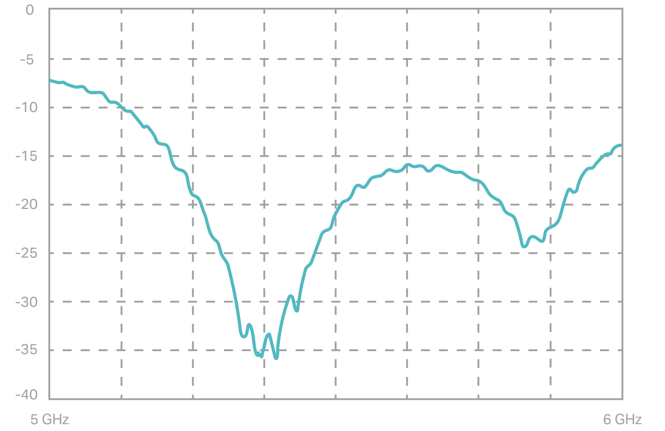
Return Loss
