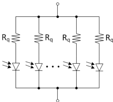
Figure 1: AFBR- S4N66C013 Block Diagram
