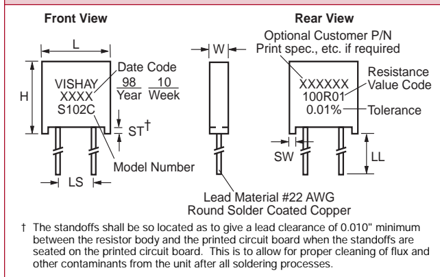
FIGURE 1 - STANDARD IMPRINTING AND DIMENSIONS
