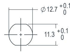
Mounting Hole
