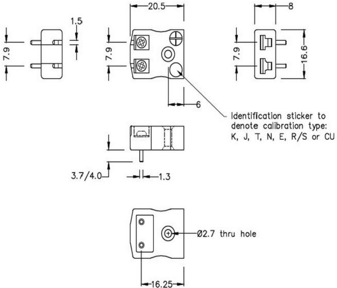
Miniature PCB Socket (dimensions in mm)
