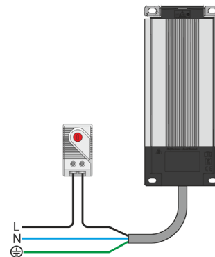
Wiring example
