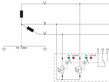
Schematic circuit diagram UL / IEC / EN
