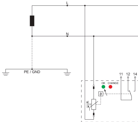
Schematic circuit diagram UL / IEC / EN
